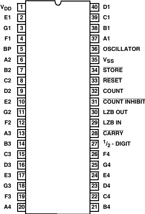
ICM7224 (PDIP) TOP VIEW
